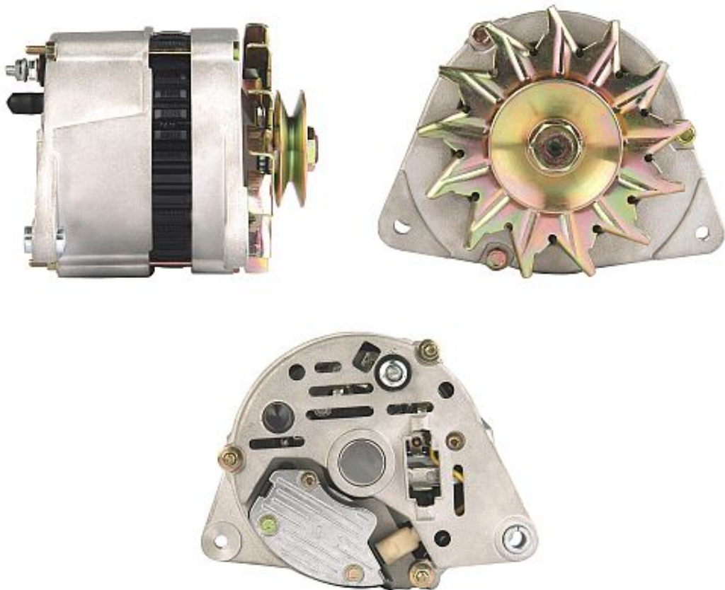
ALTERNATOR 12V,70A
